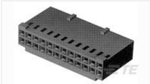
TE 产品编号280366 AMPMODU II REC. HSG DUAL ROW, 16 POS.
