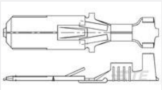
TE 产品编号42241-2 FF 250 TAB 18-14 AWG .032 TPBR
