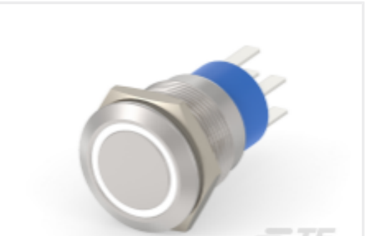
TE 产品编号4-2213767-3 AV19 DPM 3A MOVE RING LED WHITE 24V
