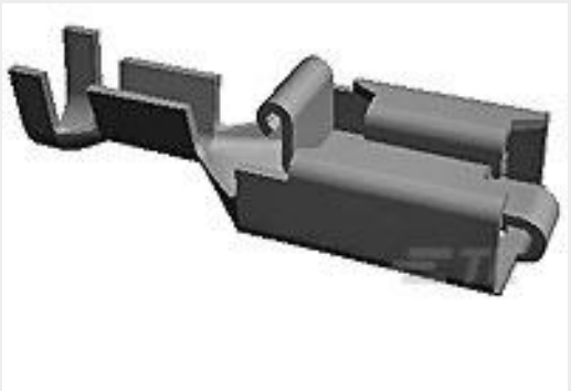
TE 产品编号154718-7 PL 250 REC TERMINAL 18-14 AWG PTPPB
