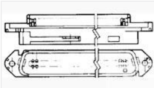
TE 产品编号552390-1 ASSY, PLUG, 50 POS, E SLOT
