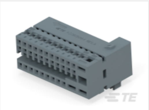
TE 产品编号1-2292506-1 34POS,MQS,REC HSG,AND MPQ
