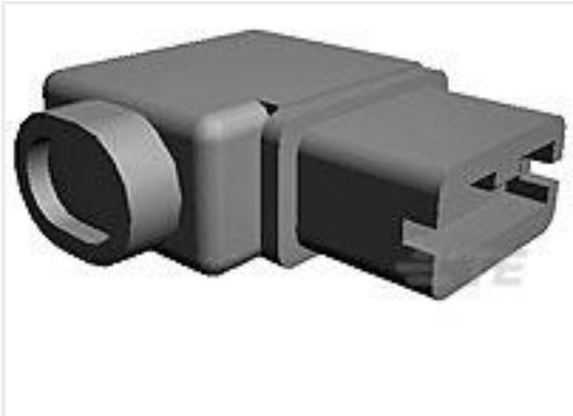
TE 产品编号1-176497-7 PL EX SLEEVE 250 FLAG RED 6/6 NYLON
