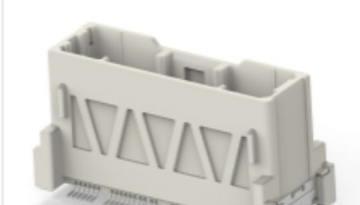
TE 产品编号2295435-9 36POS, HYBRID, HDR ASSY, 180DEG, SMD
