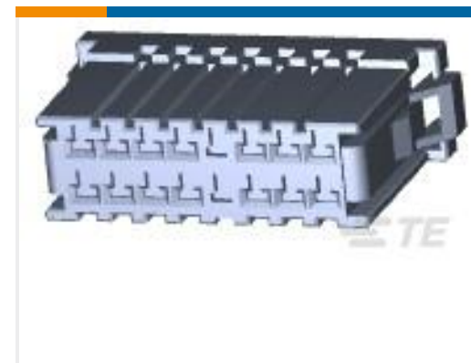
TE 产品编号178289-7 DYNAMIC D3100 REC HSG 16P
