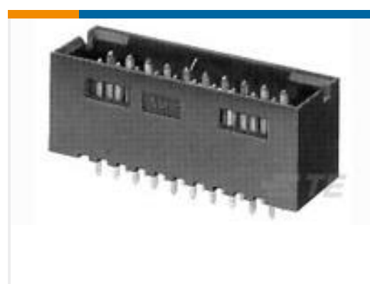
TE 产品编号5-103169-8 20 MODII HDR DRST SHRD .100CL
