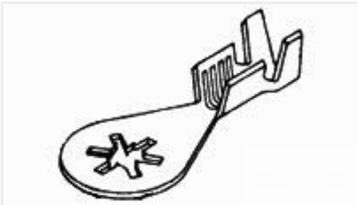
TE 产品编号62612-1 RING .164 12-10 AWG 0245 SST
