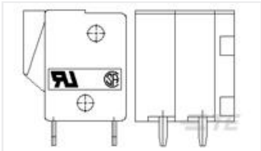
TE 产品编号1776259-4 4P Spring TB, 180deg, VT,5mm, Green
