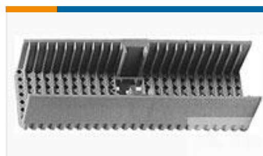
TE 产品编号646482-2 2MM H.M.,B-22 SHROUD 3.9MM
