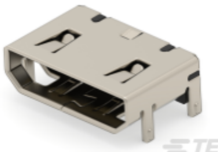
TE 产品编号 2494824-1 MiniHdmi,smt,Gold 15u,copper shell, label
