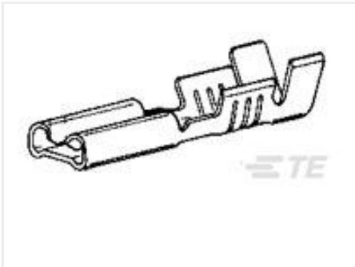
TE 产品编号170056-2 110 FASTON,REC.,24-20 AWG,TPBR
