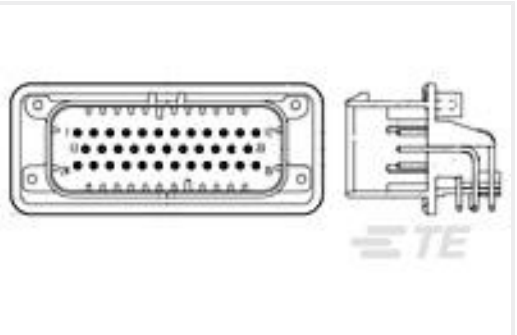
TE 产品编号776163-1 35POS,PIN DIA 1.3,HDR ASSY,90DEG, COD 1
