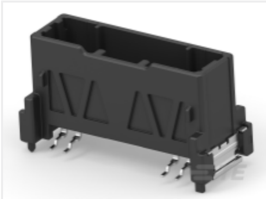
TE 产品编号1-2295435-2 36POS,HYBRID,HDR ASSY,180DEG, SMD
