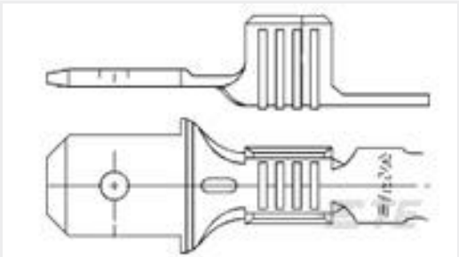
TE 产品编号63919-1 187 FASTON TAB 18-14 AWG TPBR
