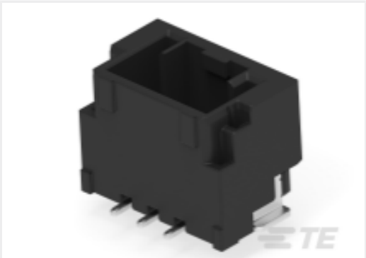
TE 产品编号2-2360547-3 SGI 1.5 HDR, 3P, VT, Key B, Black
