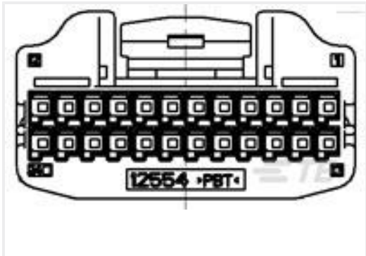
TE 产品编号1717112-1 0.64 III 24POS PLUG ASSY
