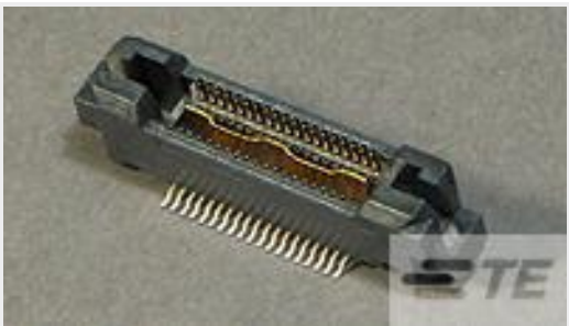
TE 产品编号5767056-1 MICT,260,PLUG,38,ASSY,PDNI
