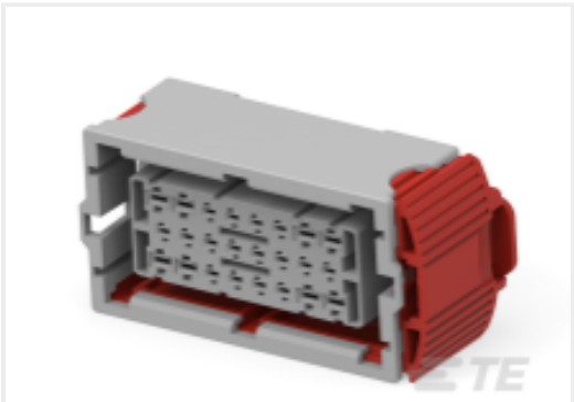
TE 产品编号1745043-3 24pos MCP hybrid conn. all ope
