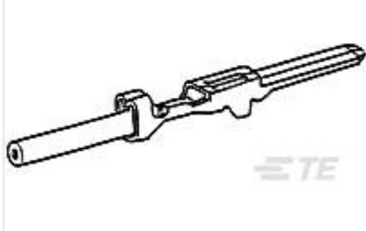
TE 产品编号173633-1 TAB CONT. (SIGNAL) AWG#22-24
