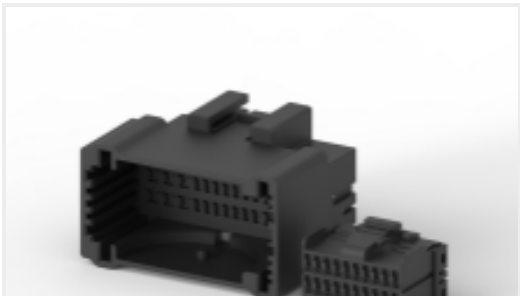
TE 产品编号520973-2 ULTRA-POD 187 ASSY REC 20-16 AWG TPBR
