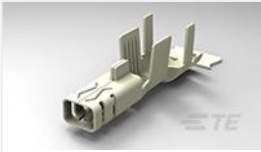
TE 产品编号5-160433-6 187 FASTON REC 20-16 AWG TPBR
