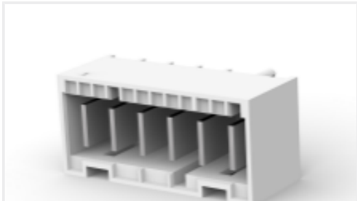
TE 产品编号1-2232532-6 6P, PL RAST 5 Tab Header, TH,Vertical
