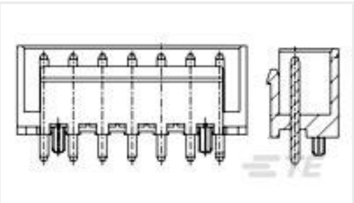
TE 产品编号1744357-7 3.96 EP SHROUDED HDR ASSY 7P W /PEGS
