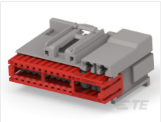
TE 产品编号1-2236269-3 24POS, MIXED, REC HSG, 20GENYMCP, ASSY, CODC
