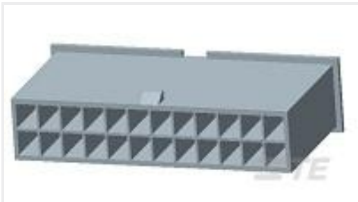
TE 产品编号521411-1 ULTRA-POD 250 ASY REC 22-18 AWG BR
