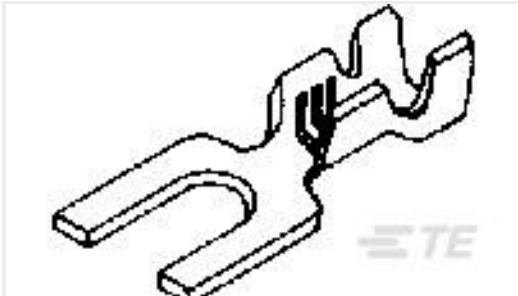
TE 产品编号60389-2 ST .138 DIA TERMINAL 20-16 AWG TPBR
