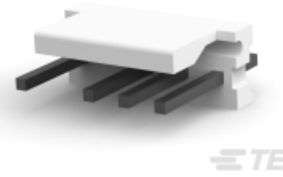
TE 产品编号643495-1 05P MTA156 HDR ASSY W/O#4
