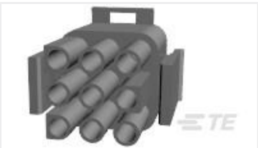
TE 产品编号1586844-1 09P UMNL PLUG HSG NATL, GW
