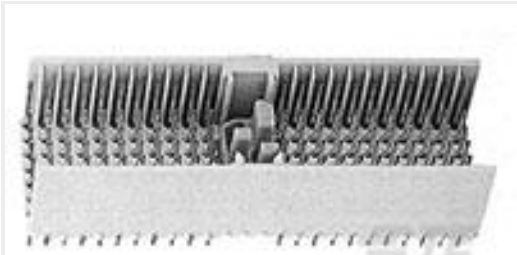
TE 产品编号5352332-1 2MM HM TYPE A MALE HDR 154 POS
