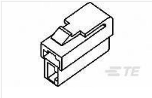
TE 产品编号172130-2 FF 250 REC HSG 2P NYLON BLCAK
