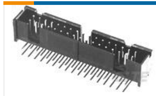
TE 产品编号5103311-5 A/L LOW PRO HDR 20P RA BLACK
