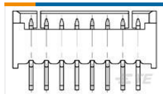
TE 产品编号2-1734598-8 1.25 WTB HDR DIP, L=2.3, 8P
