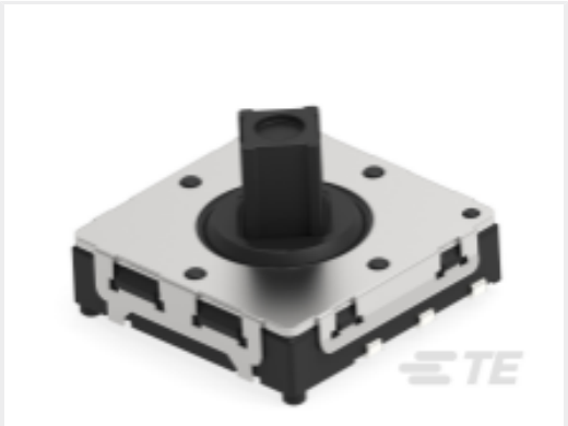
TE 产品编号2425755-1 5 position tactile, 12x12
