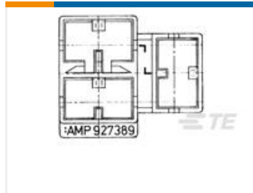
TE 产品编号927389-1 PL 3P HOUSING PA66 BLACK
