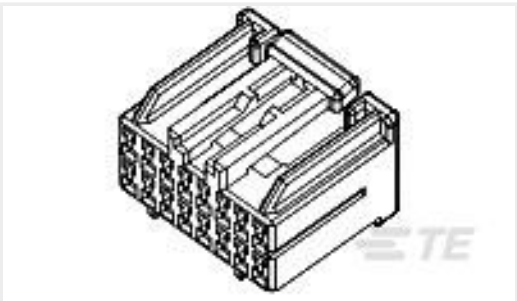
TE 产品编号917989-6 HYBRID MK-2 PLUG HSG ASSY 22P
