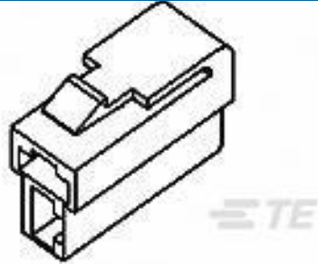
TE 产品编号172130-1 FF 250 REC HSG 2P NYLON NAT
