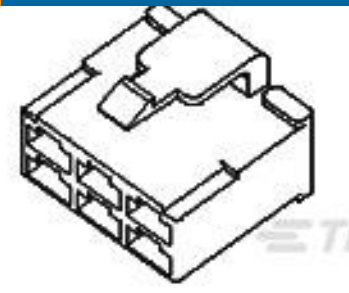
TE 产品编号172134-1 FF 250 PLUG HSG 4P NYLON NAT
