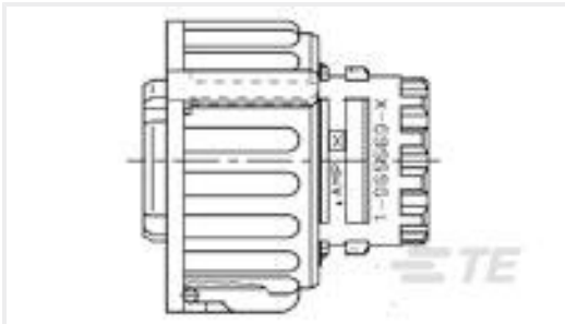
TE 产品编号1-1719434-1 4 POS DIA 2.5 SOCKET CONNECTOR HSG
