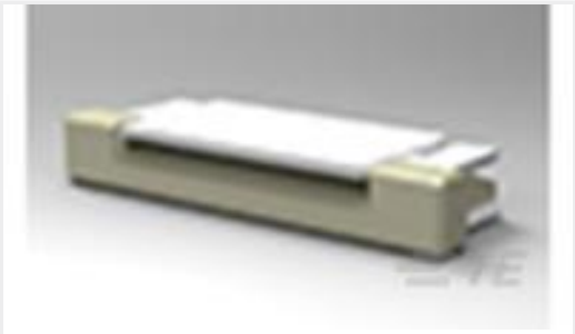
TE 产品编号1-1734839-8 FPC CONN. 0.5MM PITCH T/C,18P
