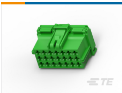
TE 产品编号1-1718491-2 AMP MCP Unsealed Connector Housings
