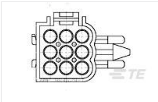
TE 产品编号964629-2 CI2 STIFT-GEH 9P
