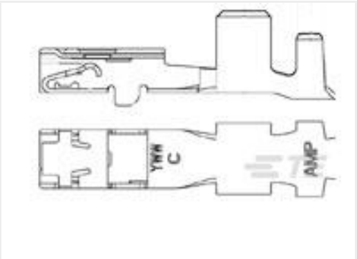
TE 产品编号1326030-6 2.8MM RECP,UNSEAL,18-20,REVREE
