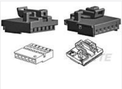
TE 产品编号284802-1 6POS MQS REC COD A
