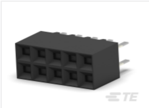
TE 产品编号2-2267056-0 40 MOIDV VRT DR CE 100/130 W/ POLARIZ
