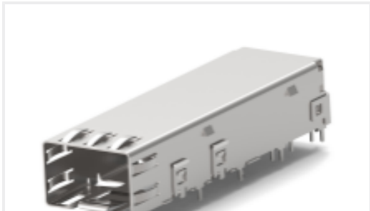
TE 产品编号1-2227303-2 CAGE ASSEMBLY, SFP, .071 TAIL
