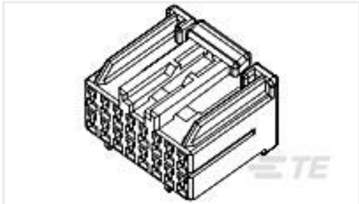
TE 产品编号 917992-6 HYBRID MK-2 PLUG HSG ASSY 26P
