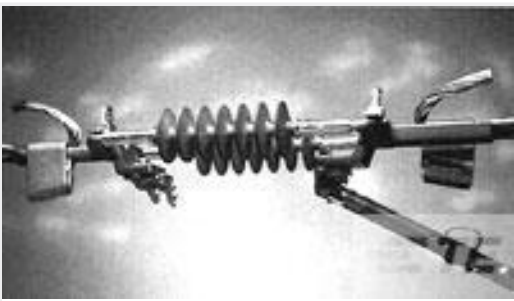
TE 产品编号83843-7 AMPACT ILD Replacement TAP 4/0
