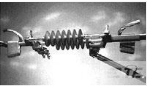
TE 产品编号83843-2 AMPACT ILD Replacement TAP 336.4
