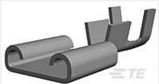
TE 产品编号160807-2 250 FASTON,REC.,20-16 AWG,BR
