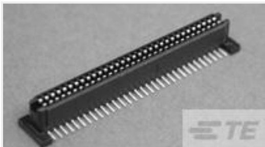
TE 产品编号5120528-1 1FHR,64,30A/S,N,C,S08,09,10
